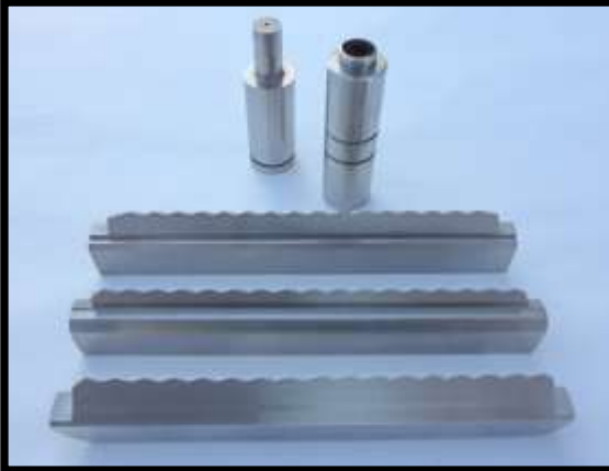
SLIT BLADES, PIERCE PUNCHES, DIE INSERTS
